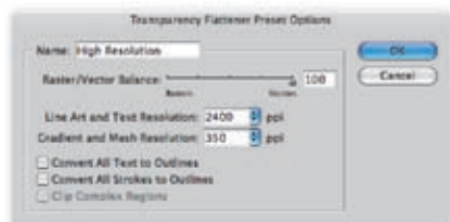
InDesign CS3 screenshot
